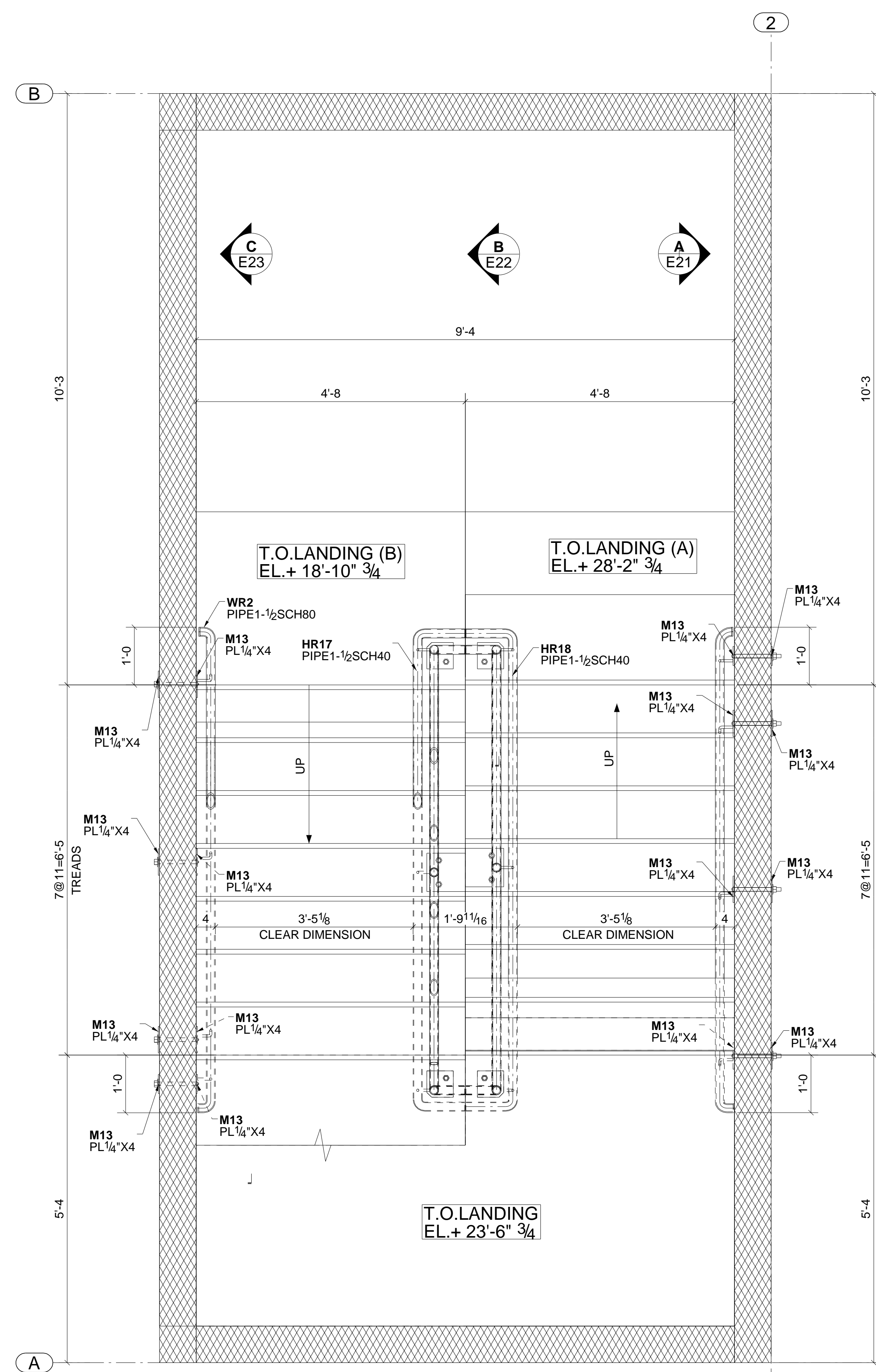
STAIR THIRD FLOOR PLAN REF DWG: 2 / TT101
