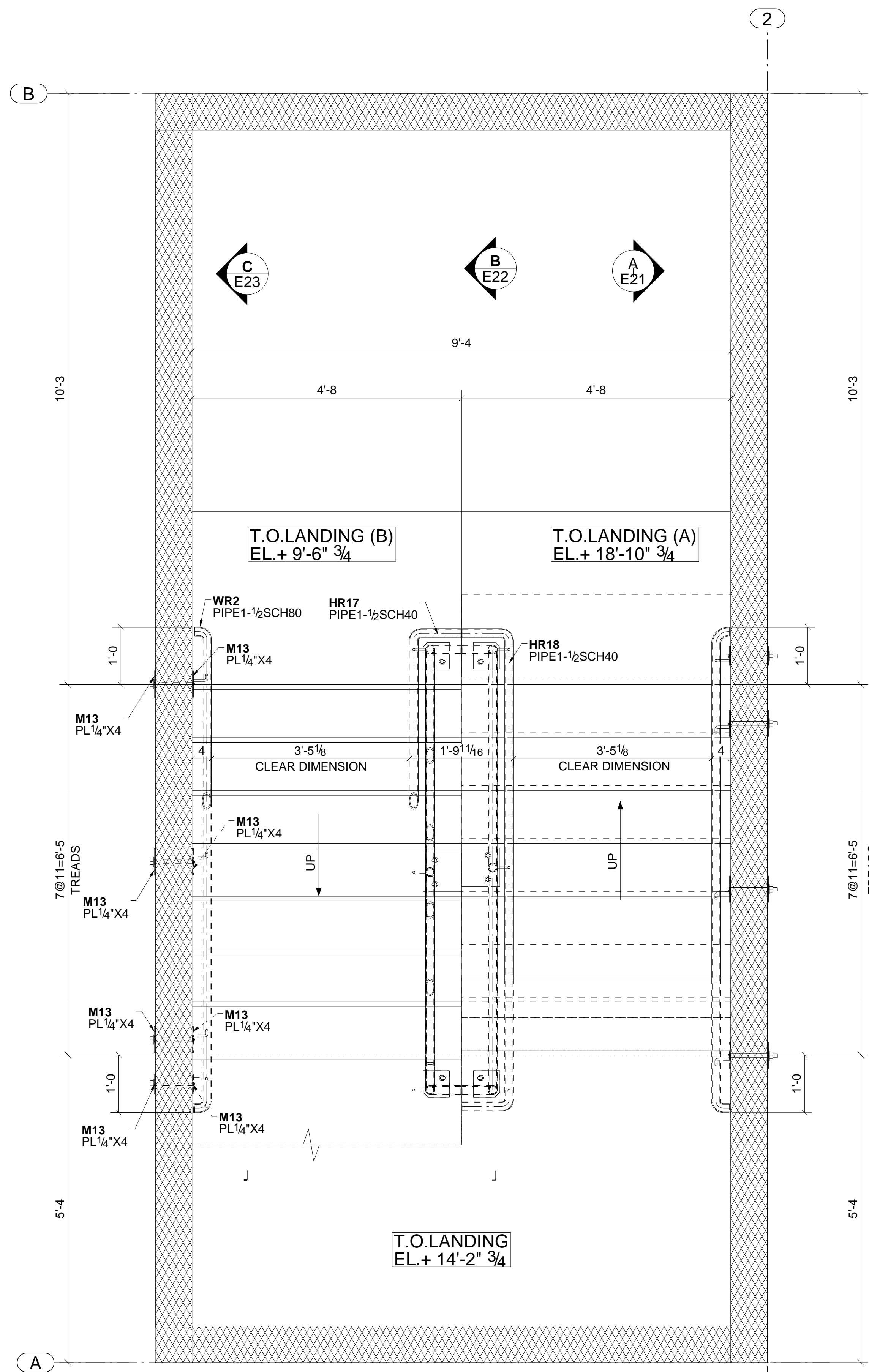
STAIR SECOND FLOOR PLAN REF DWG: 1 / TT101
