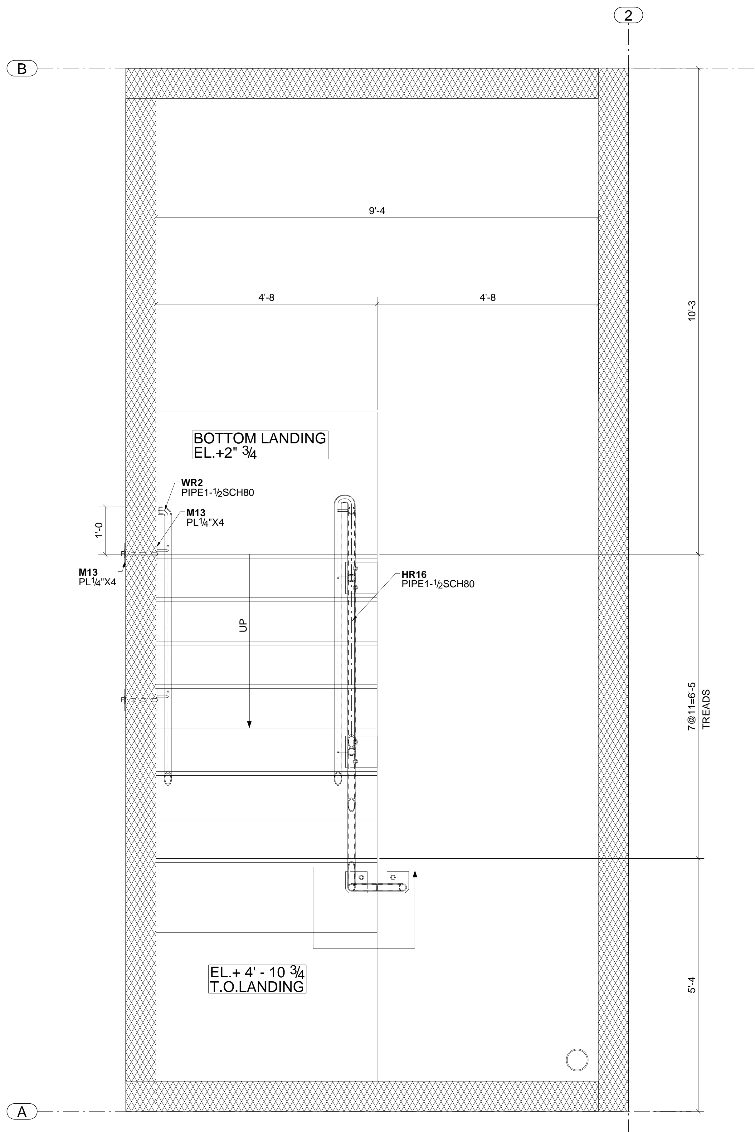
STAIR GROUND FLOOR PLAN REF DWG: 1 / TT100
