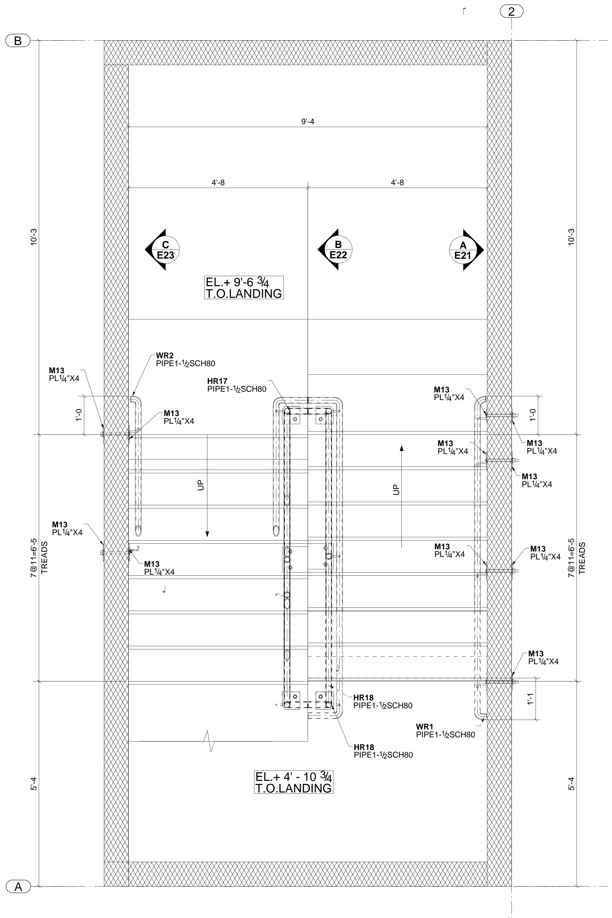
STAIR FIRST FLOOR PLAN REF DWG: 2 / TT100
