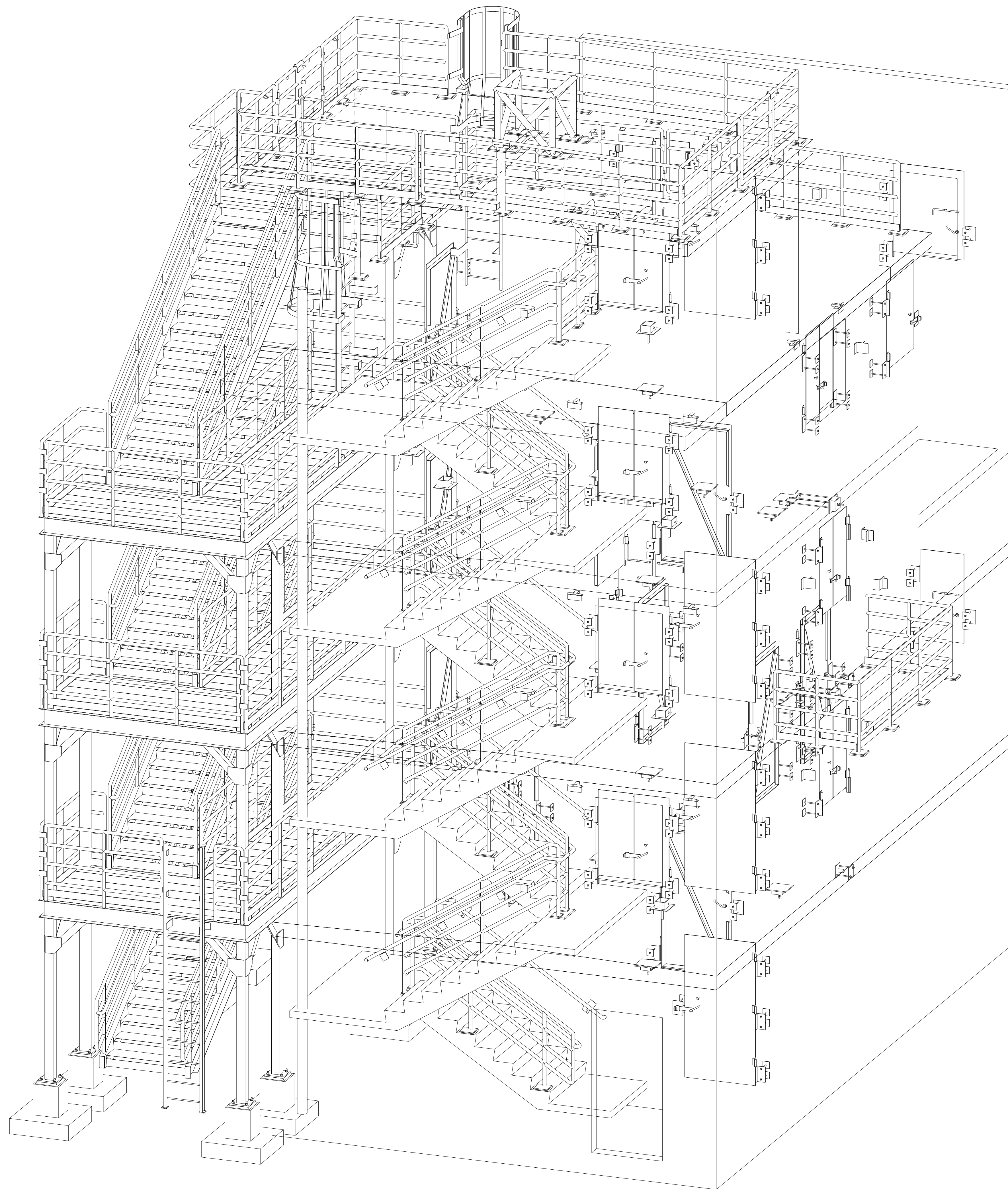
ISOMETRIC VIEW
