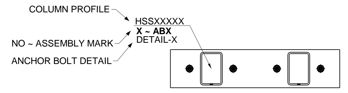
ANCHOR BOLT LEGEND
