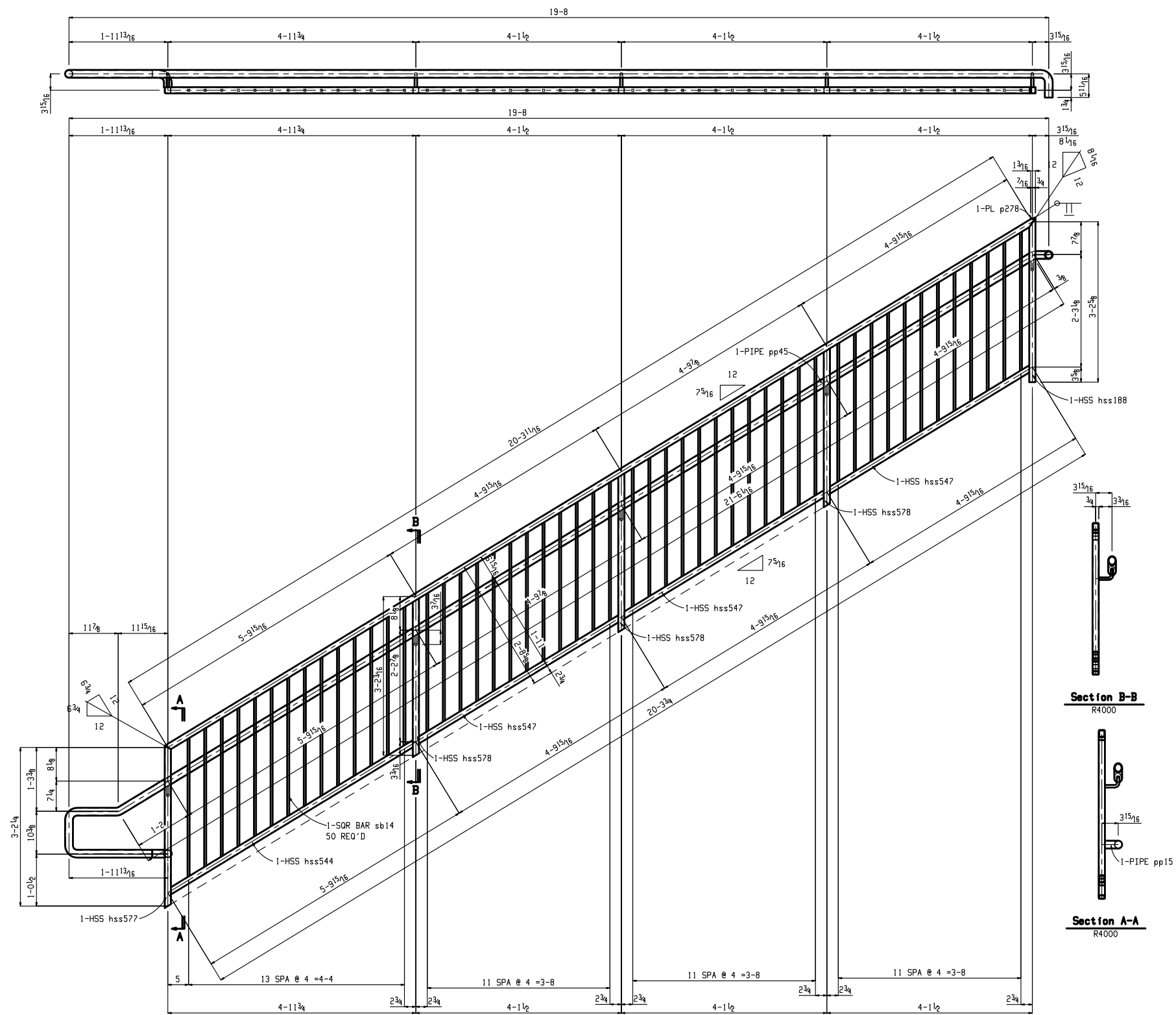
ONE HANDRAIL R4000
