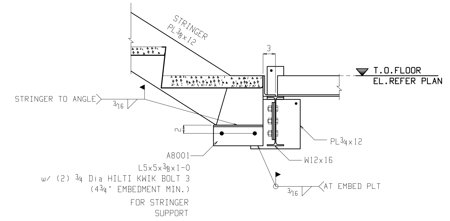
TYPICAL CONNECTION DETAIL - AA
