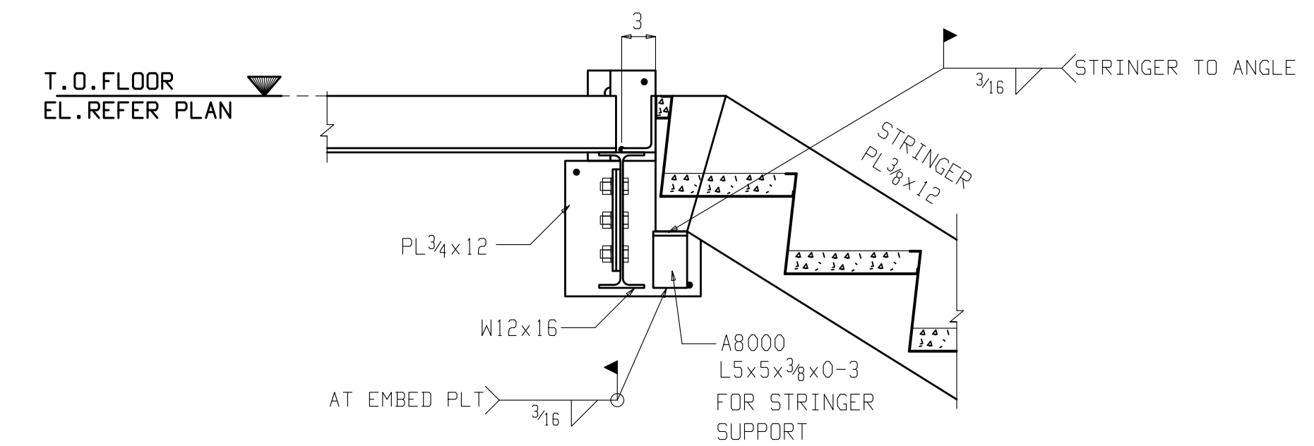
TYPICAL CONNECTION DETAIL - DD
