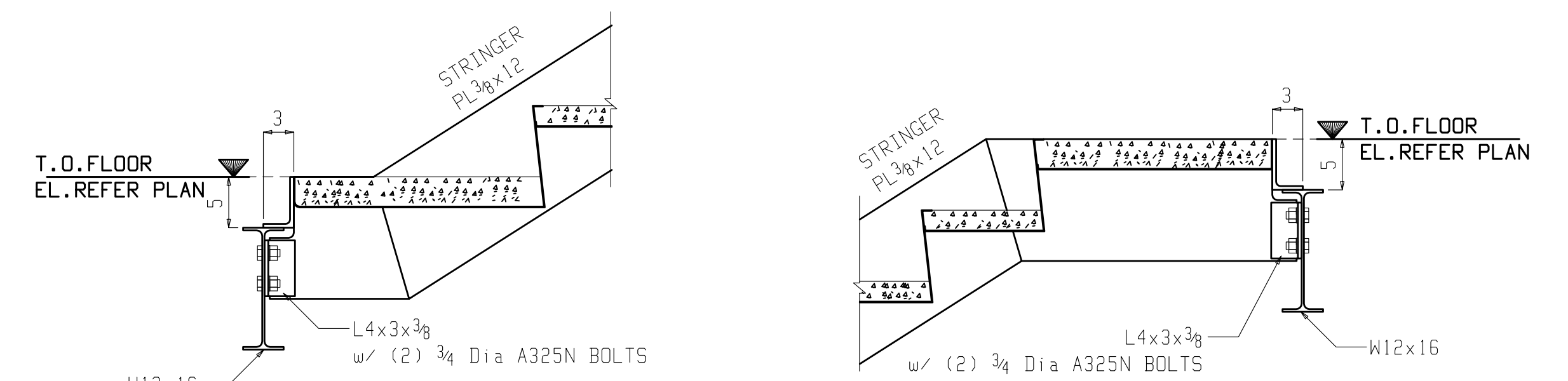
TYPICAL CONNECTION DETAIL - BB
