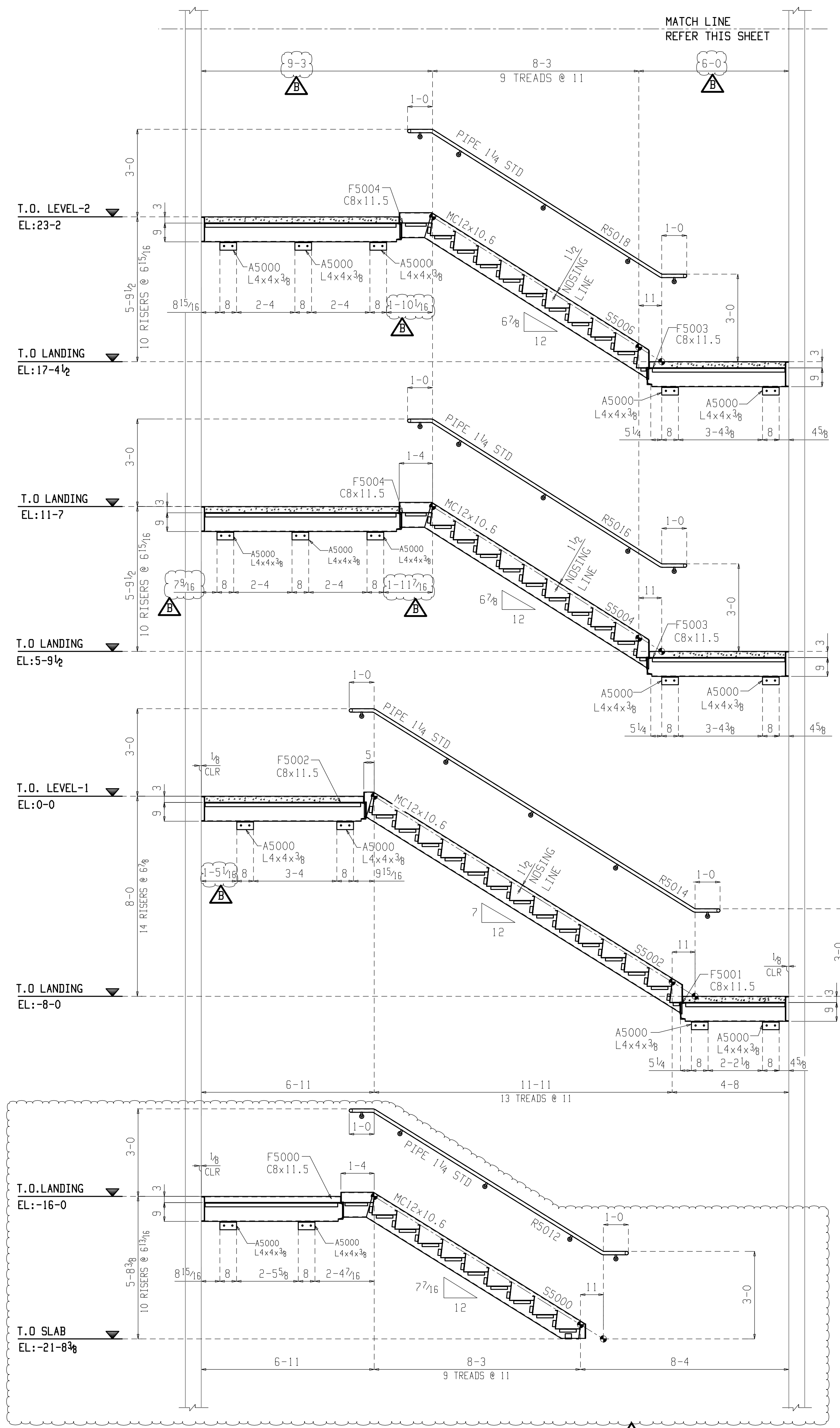
1 SECTION VIEW E5004
