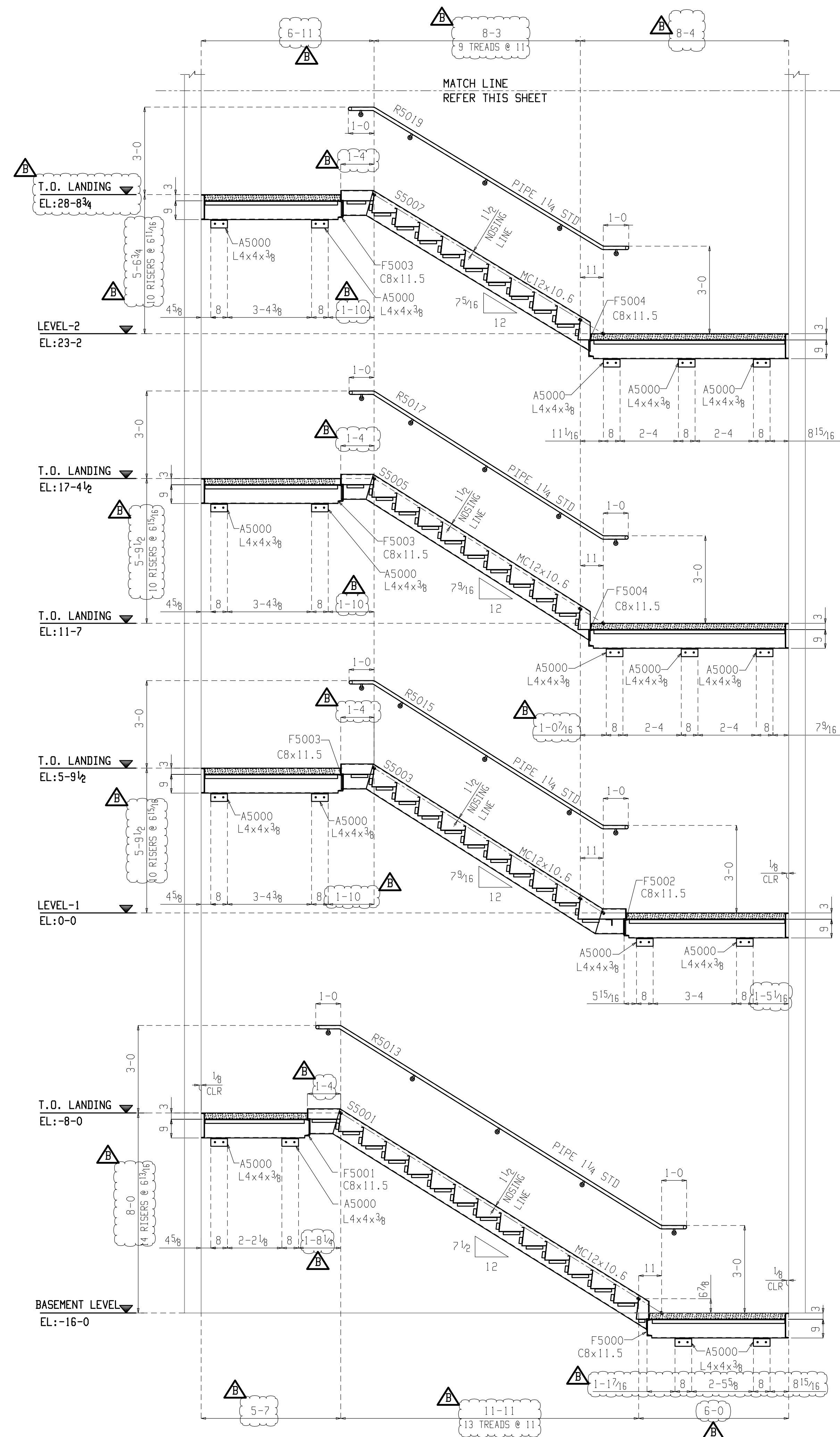
1 SECTION VIEW E5003
