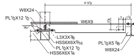
E - E Ref-section. 6/S-122
