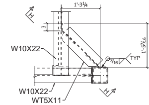
DETAIL 3 E3 Ref-section. 7/S-122
