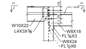
TYPICAL MOMENT CONNECTION DETAIL E3
