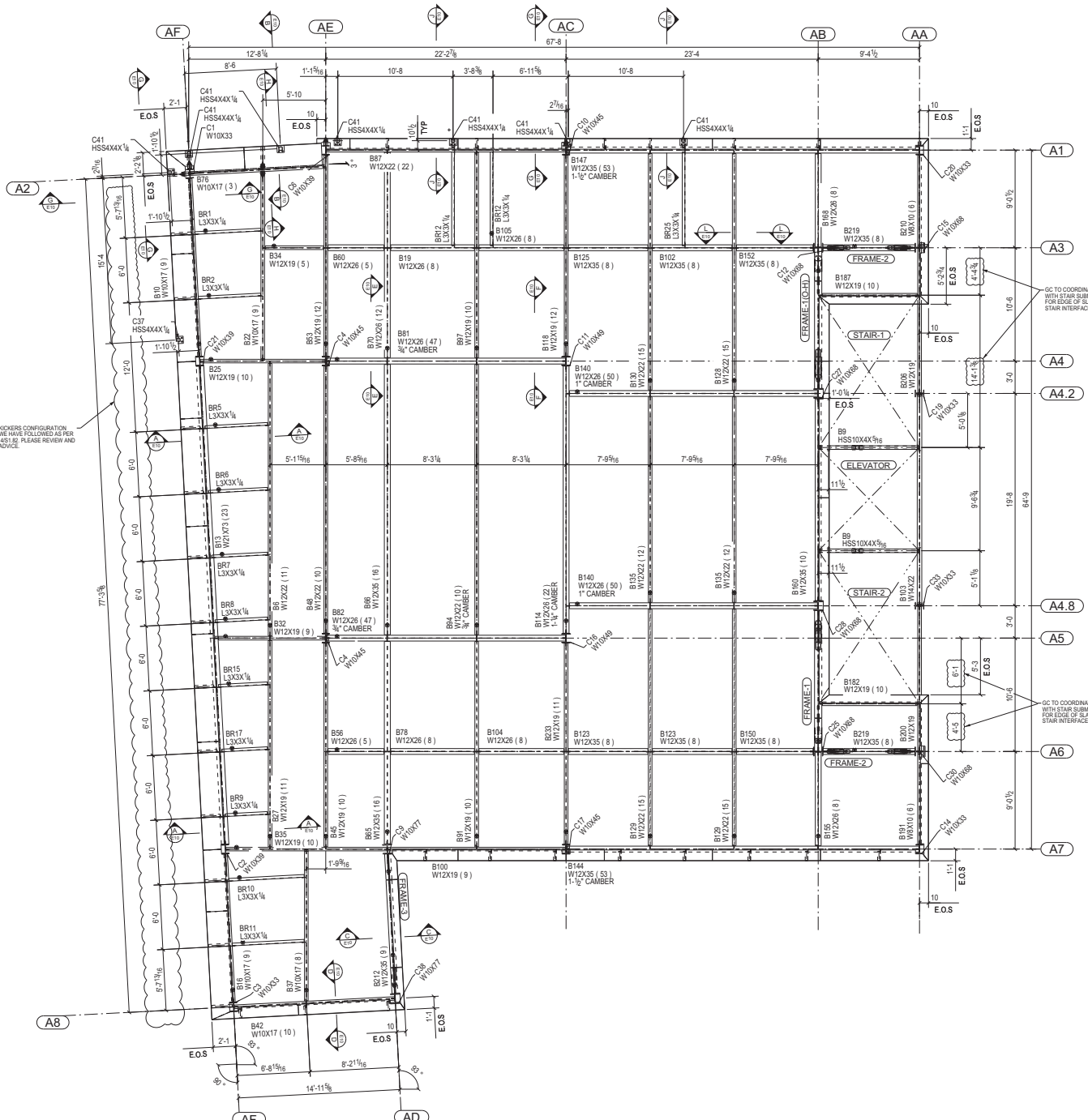
SECOND LEVEL FRAMING PLAN T.O.S EL. + 16'2 3/4 (U.N.O) Ref: 2/S2.81 & 2/A11.81
