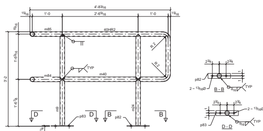
ONE - HANDRAIL - 40HR2
