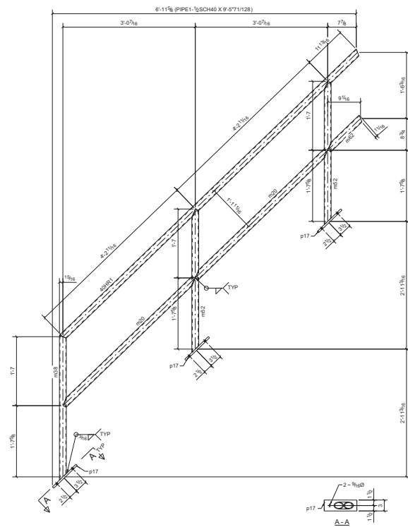
ONE - HANDRAIL - 40HR1
